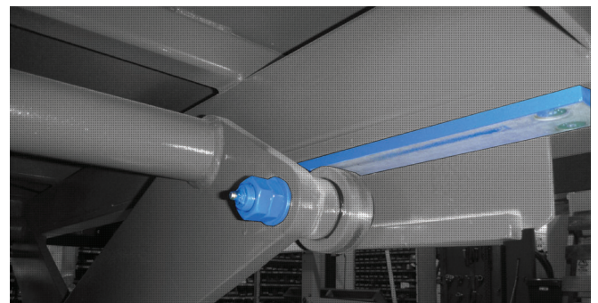
Greasable Roller followers and Bisalloy 80 roller paths upper & lower
