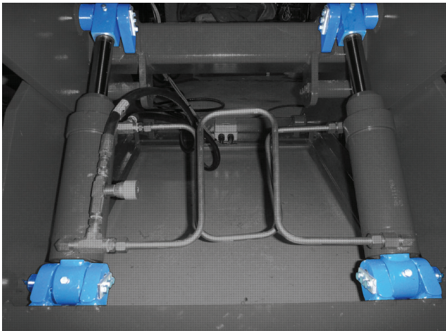
Cylinder hinge ends Include greasable pivots *not available on all models
