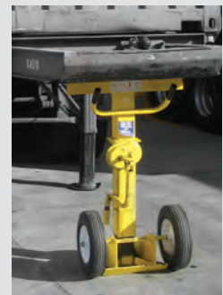
In secure supporting position. Trailer can now be safely loaded.
