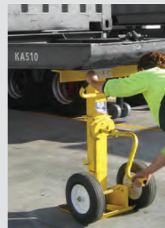
Winding up into secure supporting position
