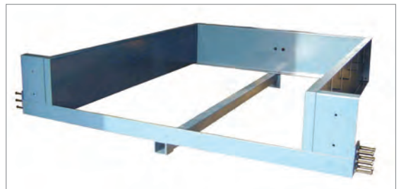
Ezi-Pit suitable for Standard or Tail Lift Provision Docks can be provided to assist in pit formation during loading dock construction
