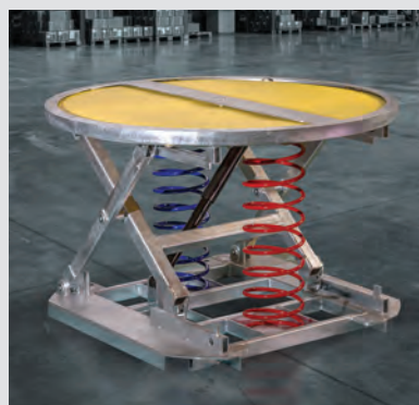
PTG3 with rotating top
